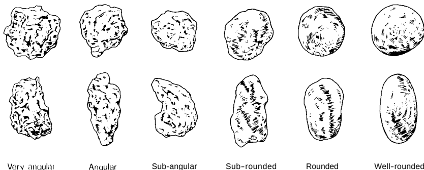
13 Diagram to show degrees of roundness in the shape of pebbles (redrawn after Powers 1953):
