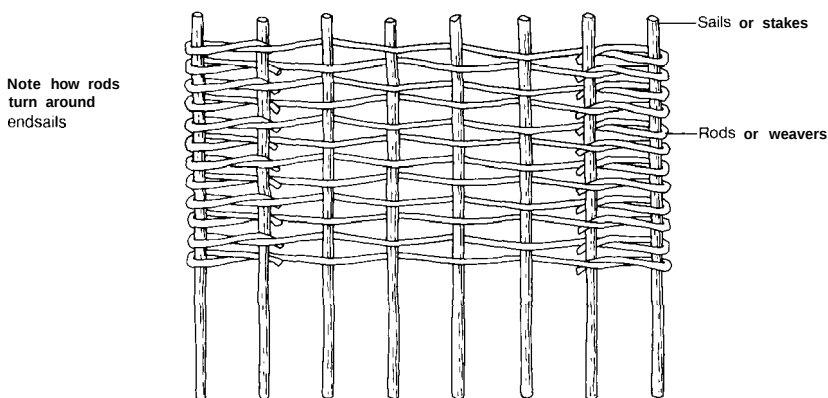
34 Diagram of a wattle hurdle.
